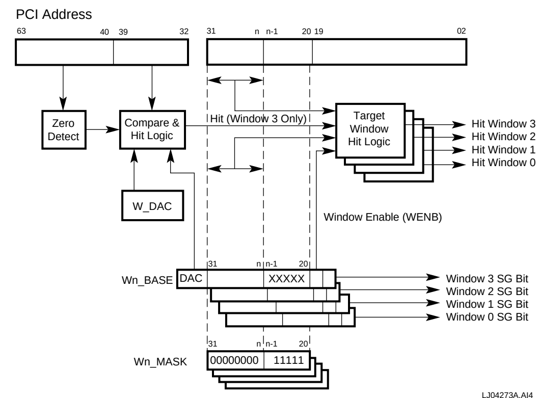
Figure 6–18 PCI Target Window Compare
