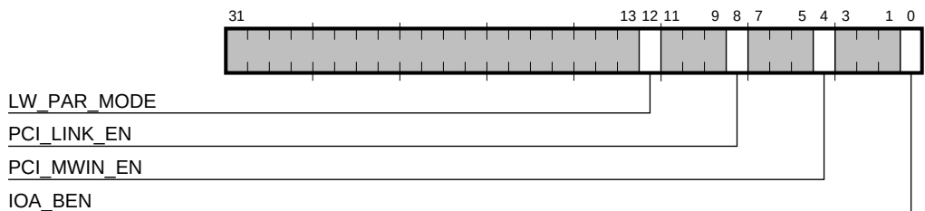
Figure 5–4 Control Register 1
