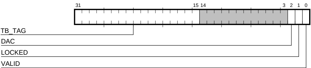
Figure 5–39 Lockable Translation Buffer Tag Register
