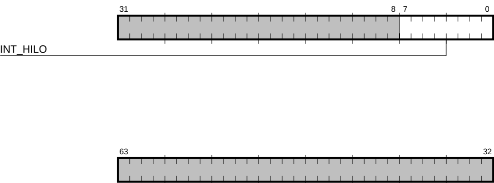
Figure 5–47 Interrupt High/Low Select Register
