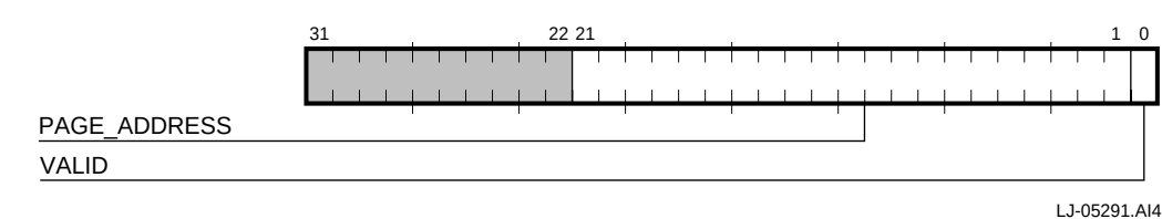
Figure 5–41 Translation Buffer Page Register
