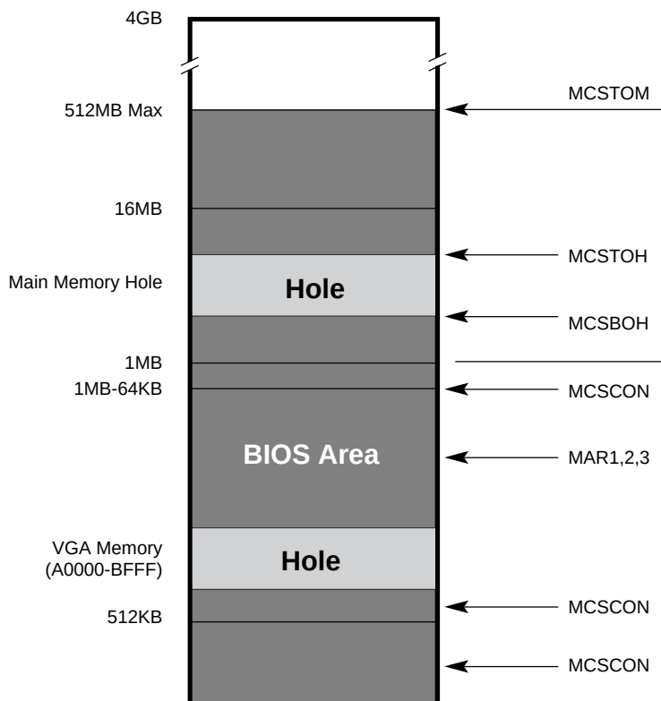
Figure 6–23 mem_cs_l Decode Area
